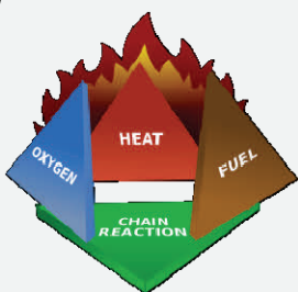
Fire Tetrahedron
